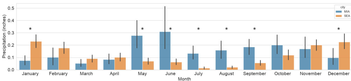
Fig(3) Precipitation for each month
