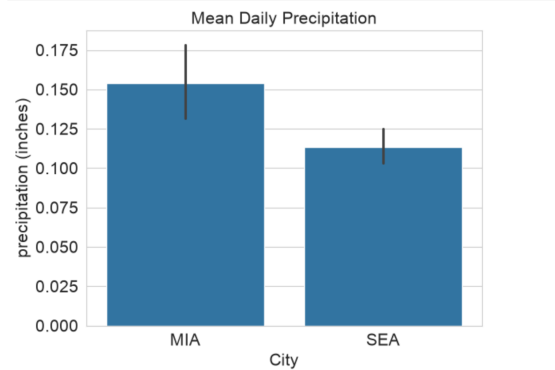
Fig(1): Mean daily Precipitation
