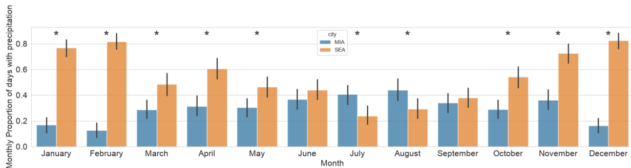
Fig(4) Monthly proportion of days with precipitation
